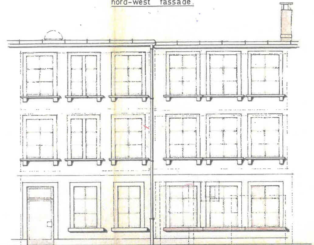
nord-west fassade.
